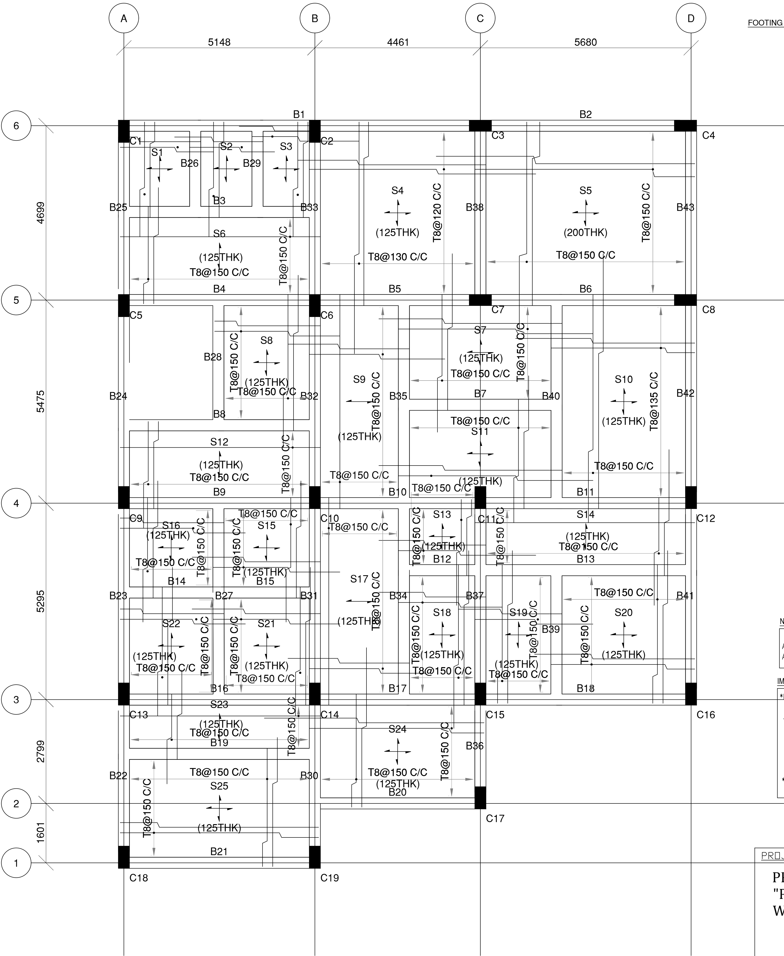
BENTUP REINFORCEMENT LAYOUT - 0 M
